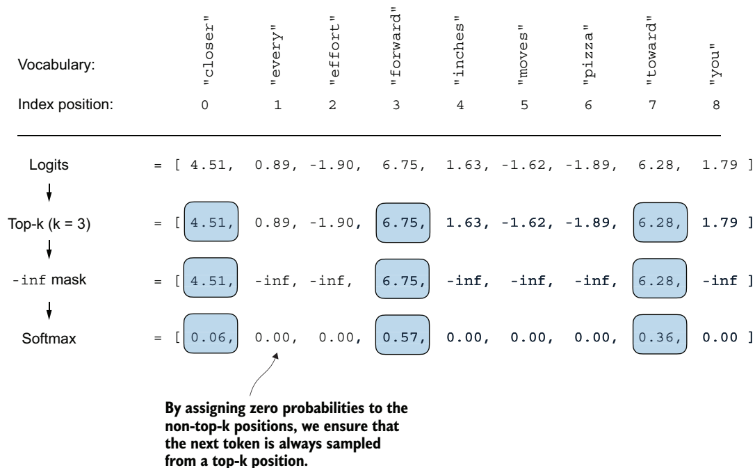
Figure 5.15 Using top-k sampling with k = 3 , we focus on the three tokens associated with the highest logits and mask out all other tokens with negative infinity ( -\text{inf} ) before applying the softmax function. This results in a probability distribution with a probability value 0 assigned to all non-top-k tokens. (The numbers in this figure are truncated to two digits after the decimal point to reduce visual clutter. The values in the “Softmax” row should add up to 1.0.)
